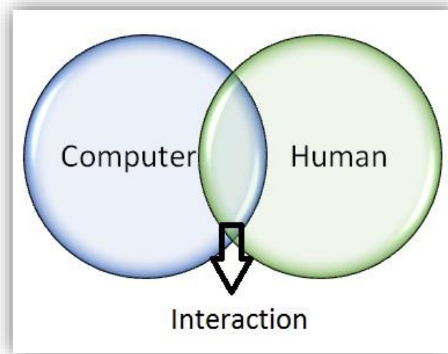
Figure 1: Human-Computer Interaction
