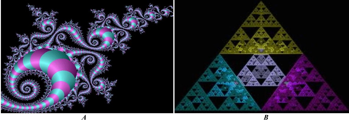
Figure 5: A) A snail like fractal geometry, B) Triangle fractal geometry.
