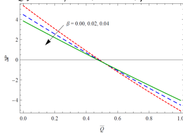
Fig. 4. \Delta P vs \bar{Q} for \beta with \phi = 0.6 , We = 0.001 , n = 0.02 and k = 1
