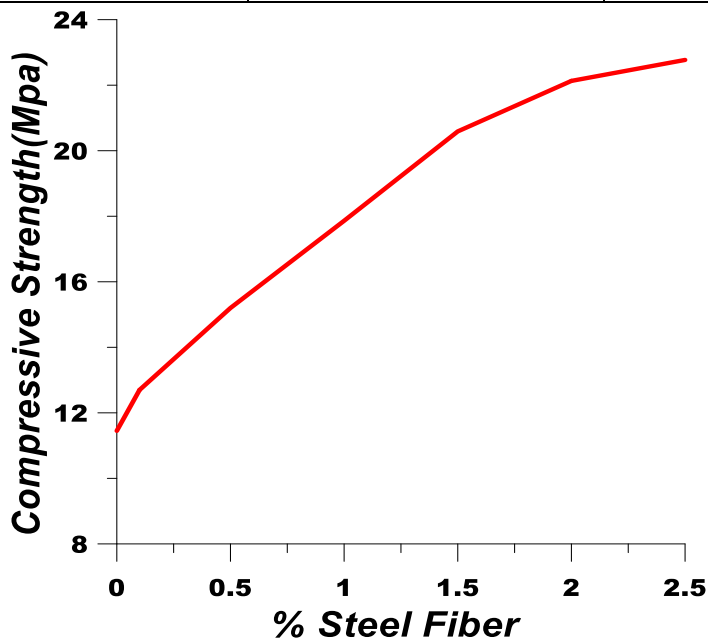
Fig. 8 Compressive Strength Test
